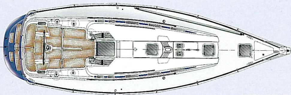
DECK LAYOUT
