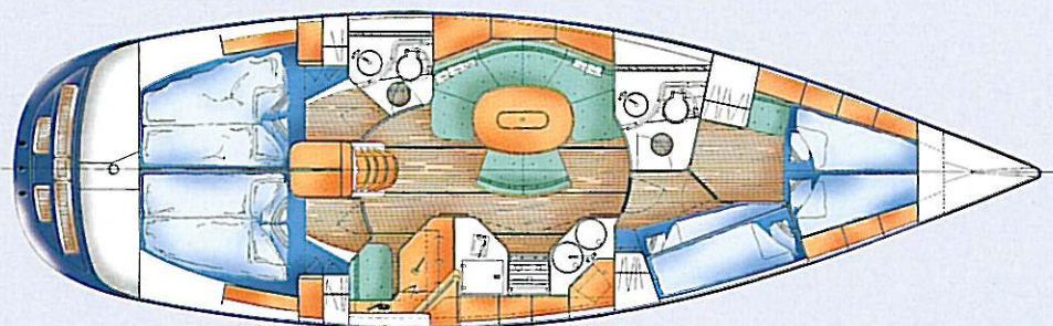
4 CABIN ACCOMMODATION
